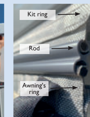
Use on a rail installed in the blind
